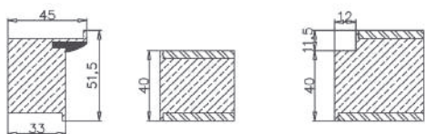
DOOR FRAME LEAF LEAF STANDART 51 TECHNOFORM 40 TECHNOFORM 51
