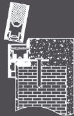
MONOBLOCK A TECHNOFORM 40
