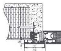
MONOBLOCK B TECHNOFORM 51
