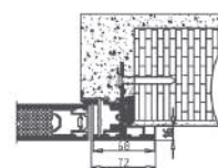
MONOBLOCK A TECHNOFORM 40
