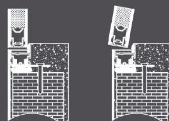
STANDART 51 TECHNOFORM 51 (WALL PANELS)
