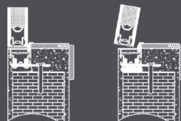
STANDART 51 TECHNOFORM 40 (MDF PORTAL FRAME)
